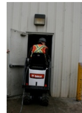
Electric Compact Excavator Fits Through A 32" Wide Opening
